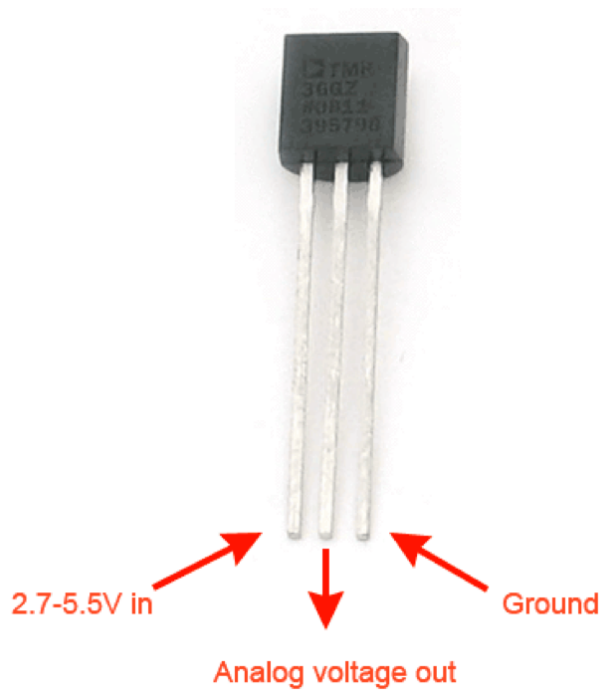
Figure 28.7: TMP36 Temperature Sensor
