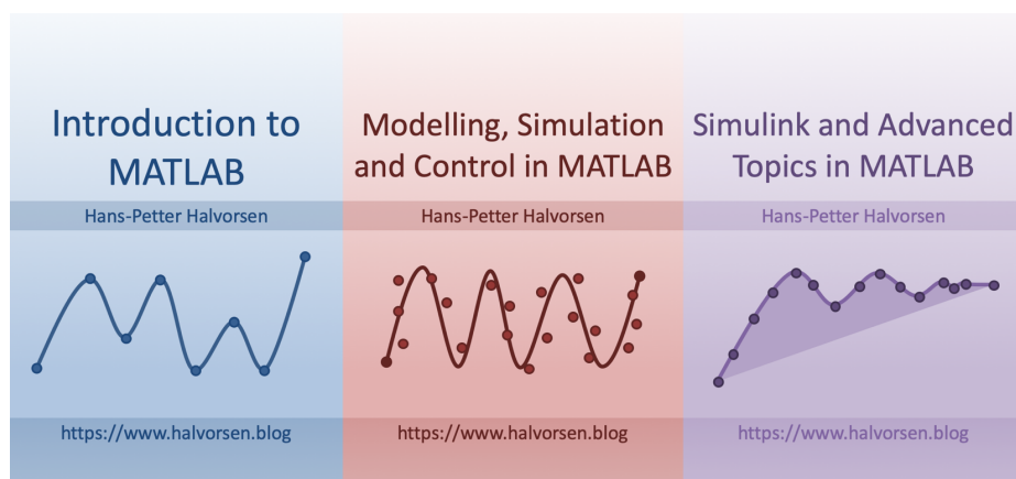
Figure 38.1: MATLAB Textbooks
