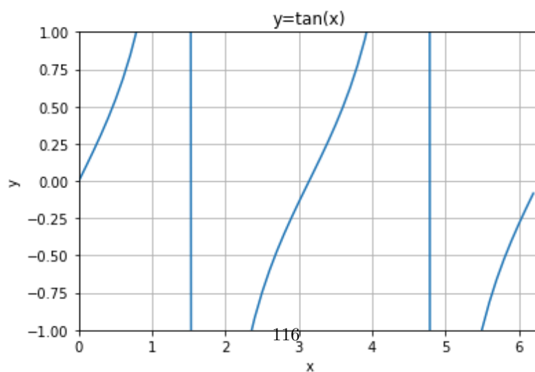
Figure 18.3: Trigonometric Functions
