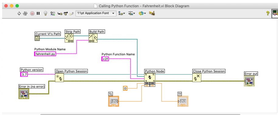
Figure 36.3: Python Integration in LabVIEW
