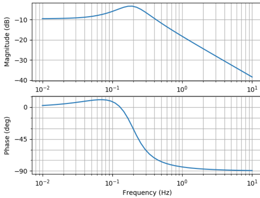
Figure 32.5: Frequency Response
