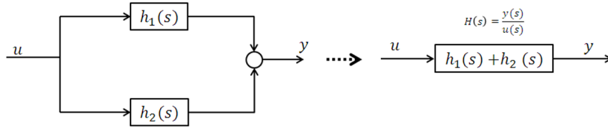
Figure 30.8: Parallel Block Diagram
