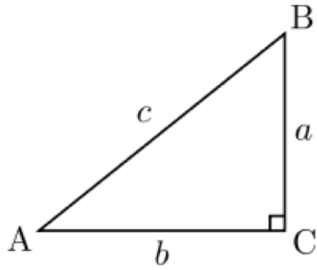
Figure 18.4: Right Triangle
