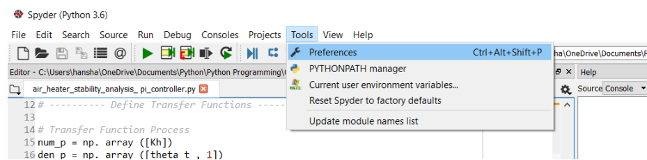
Figure 16.2: Python Tools-Preferences
